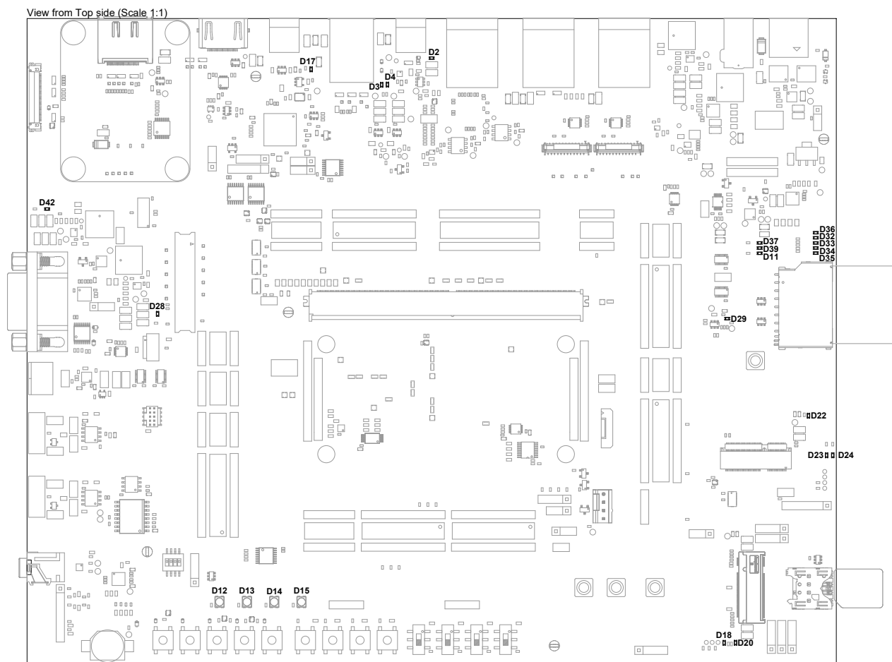
Figure 3: SMARC Development Board Indicator LEDs
