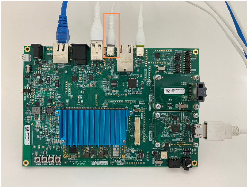
Figure 5: USB OTG Connection
