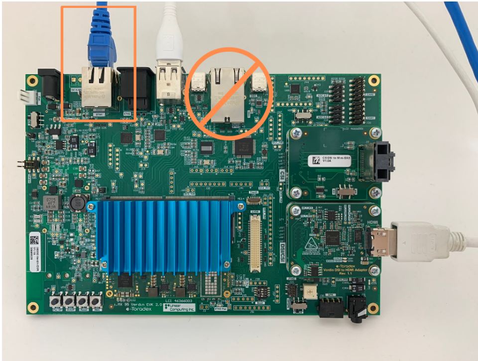
Figure 3: Ethernet Connection
