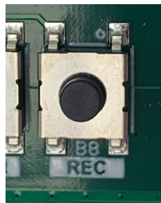
Figure 10: Recovery Button B8
