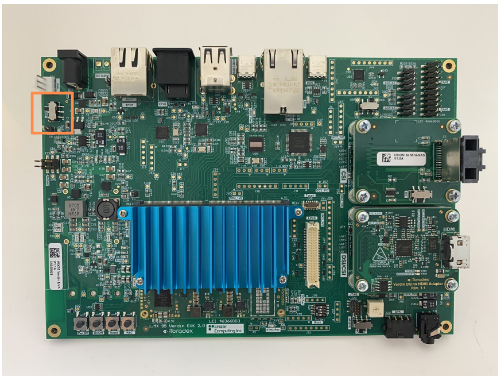
Figure 13: Location of Power On/Off Switch S6
