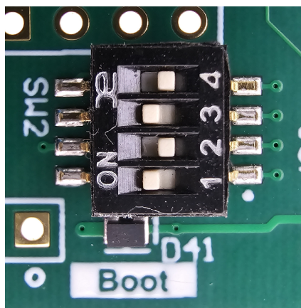
Figure 7: Dip Switch SW2 configuration
