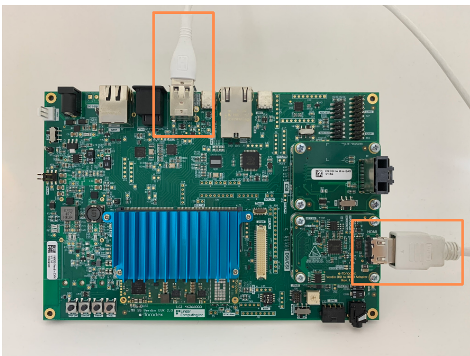
Figure 2: HDMI and Display power/touch USB Connection
