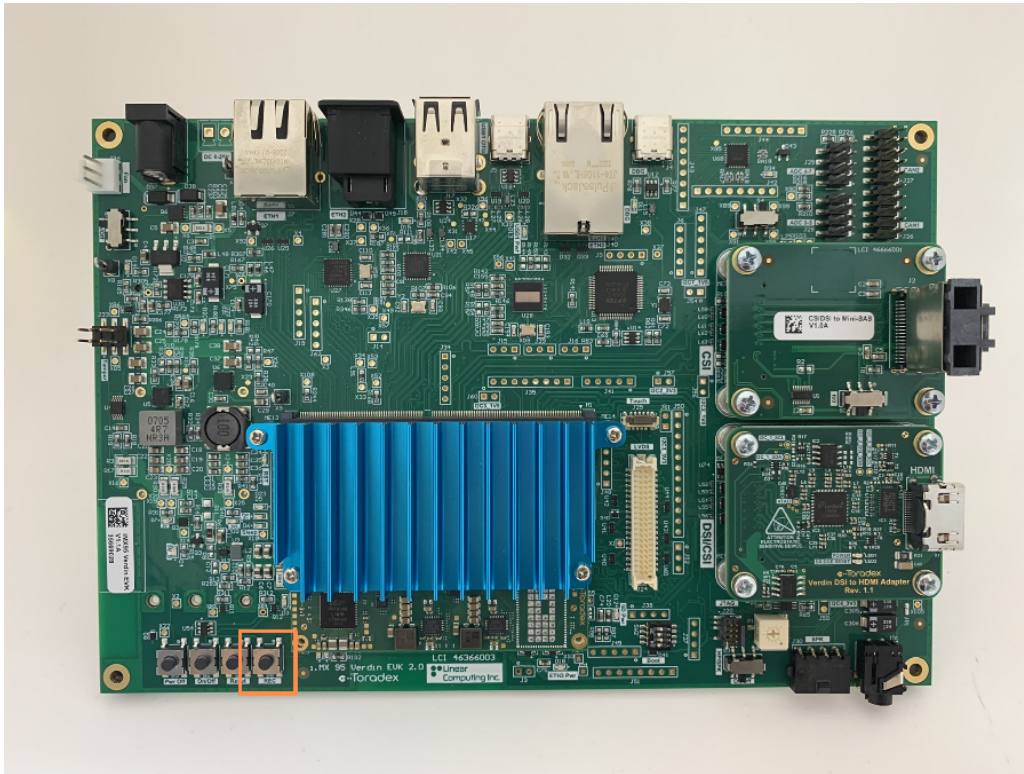
Figure 12: Recovery Button B8 location
