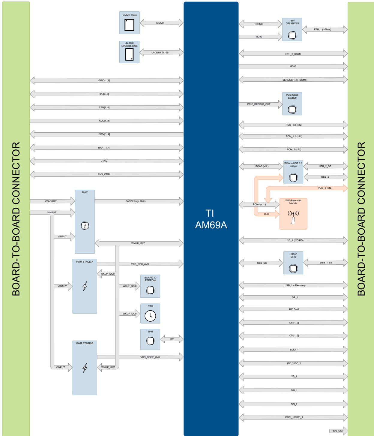
Figure 1: Block Diagram
