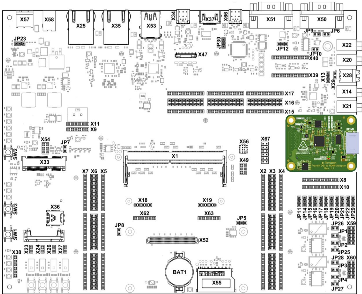
Figure 4. Toradex DSI to HDMI Adapter installed on the Verdin Development Board
