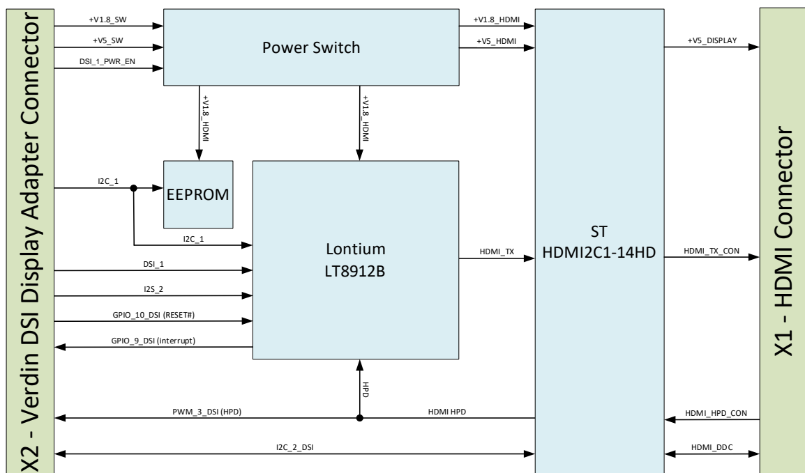
Figure 1. Toradex DSI to HDMI Adapter Hardware Architecture
