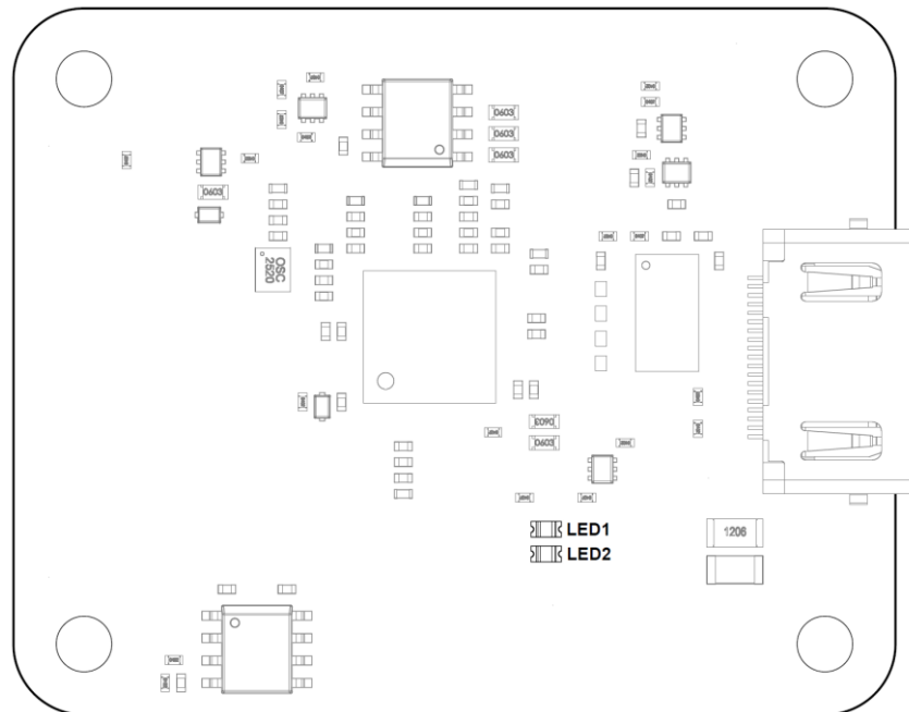
Figure 6. Toradex DSI to HDMI Adapter LEDs
