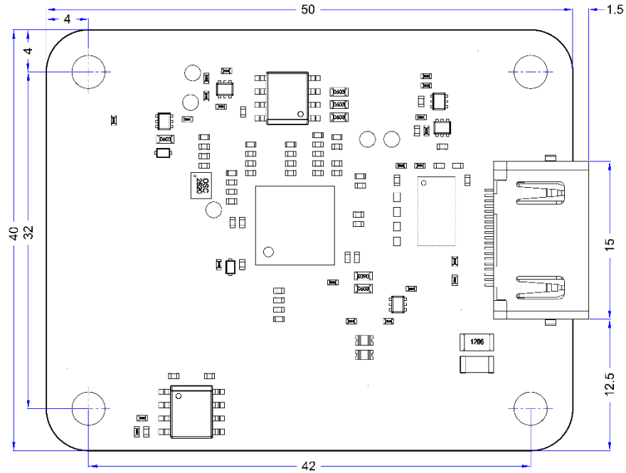
Figure 8. Toradex DSI to HDMI Adapter Dimensions in mm (top side, top view).
