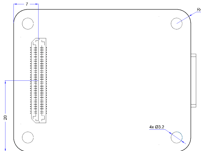
Figure 9. Toradex DSI to HDMI Adapter Dimensions in mm (bottom side, bottom view)
