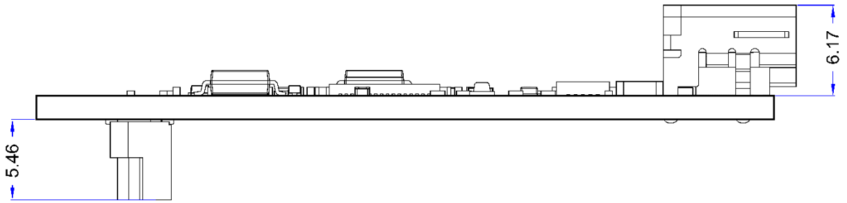
Figure 10. Toradex DSI to HDMI Adapter Dimensions in mm (side1, side 1 view).
