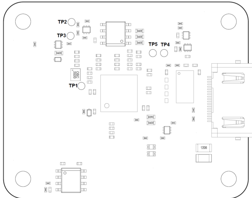
Figure 7. Toradex DSI to HDMI Adapter Test Points
