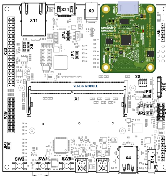
Figure 5. Toradex DSI to HDMI Adapter installed on the Dahlia carrier board
