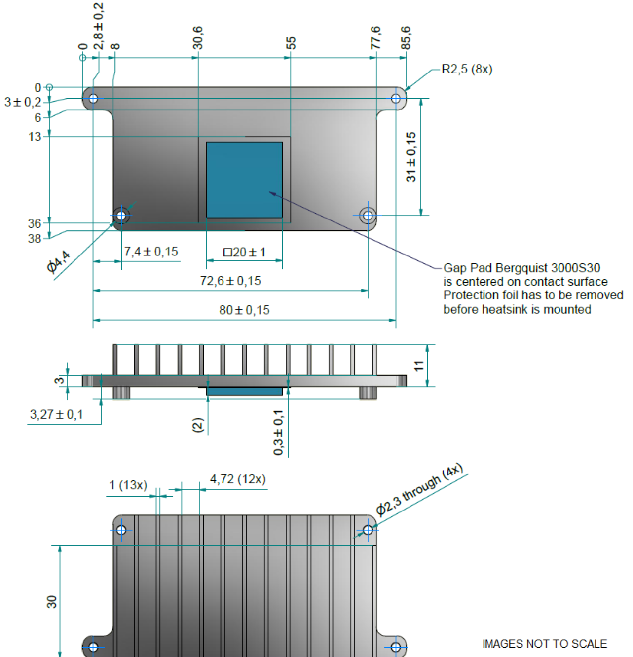
Figure 1-A: Verdin Industrial Heatsink Type 1 Dimensions
