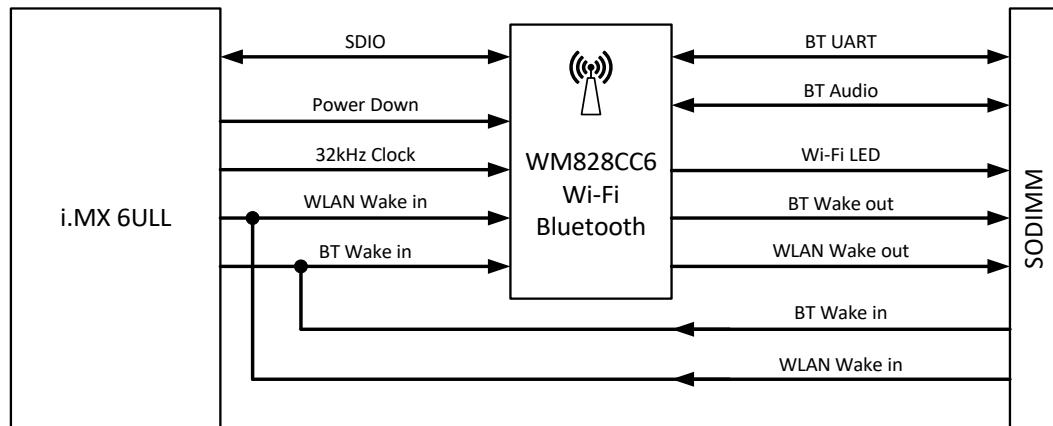
Figure 5: Wi-Fi and Bluetooth block diagram
