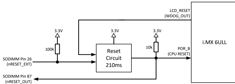
Figure 4: Reset Circuit
