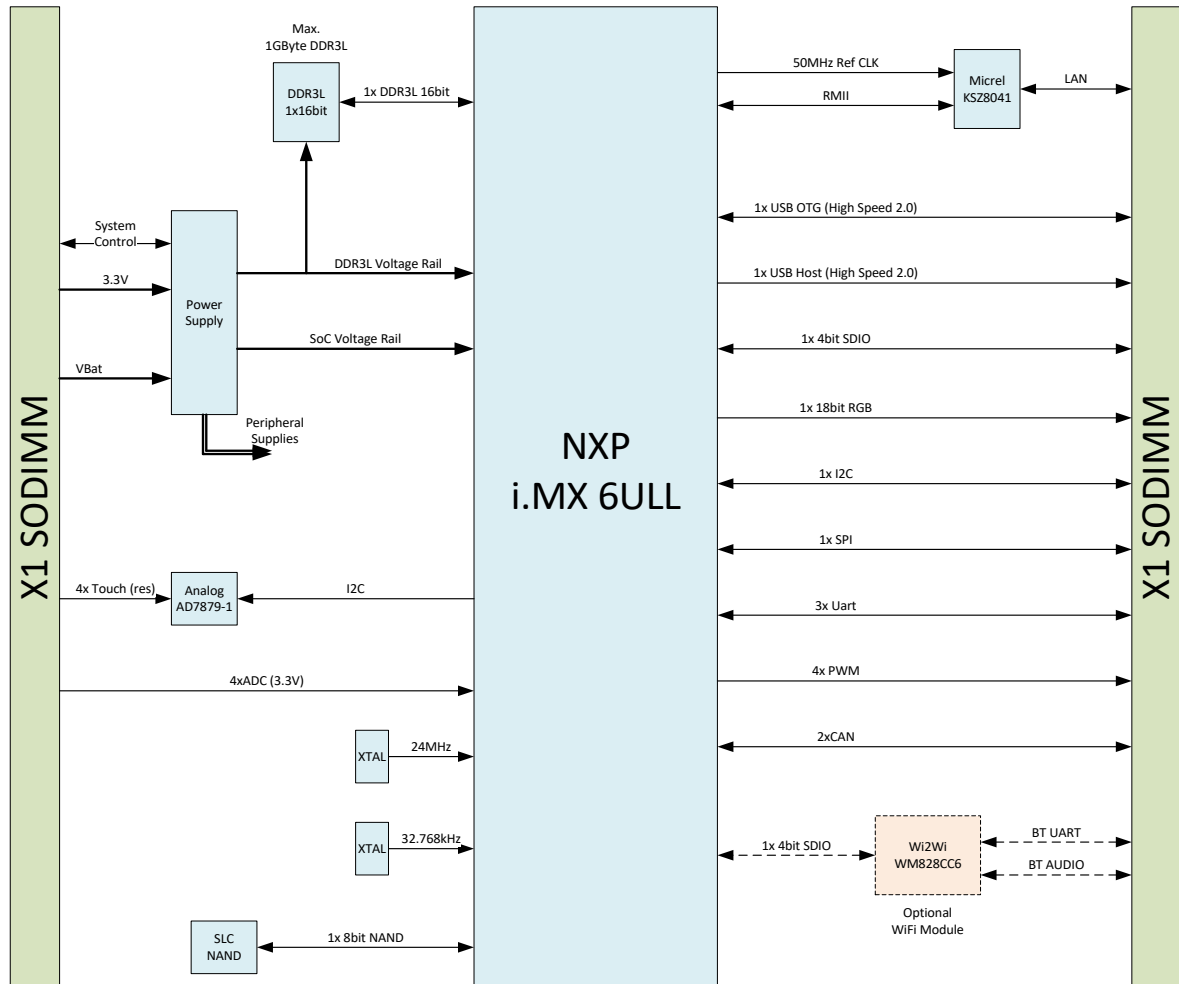
Figure 2 Colibri iMX6ULL Block Diagram
