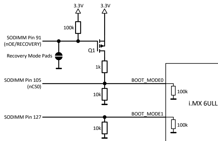
Figure 8: Recovery Mode Glue Logic
