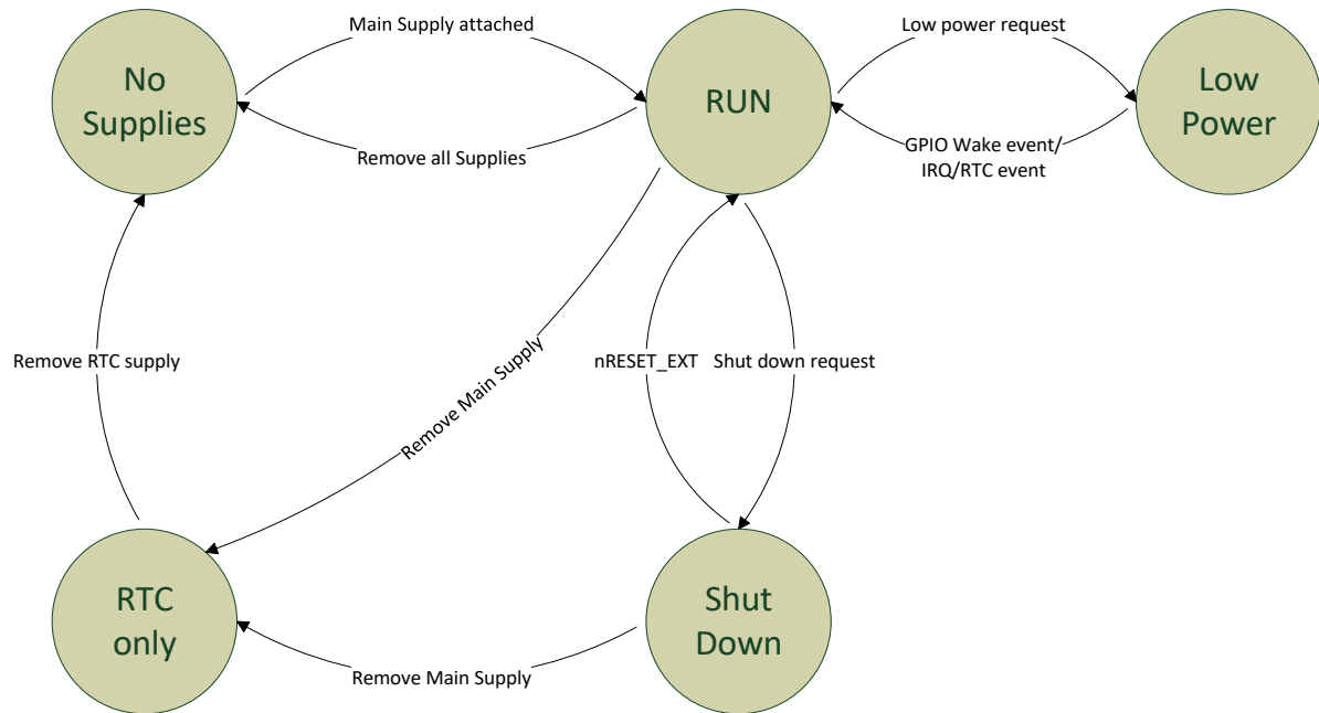
Figure 6: Run and Sleep States
