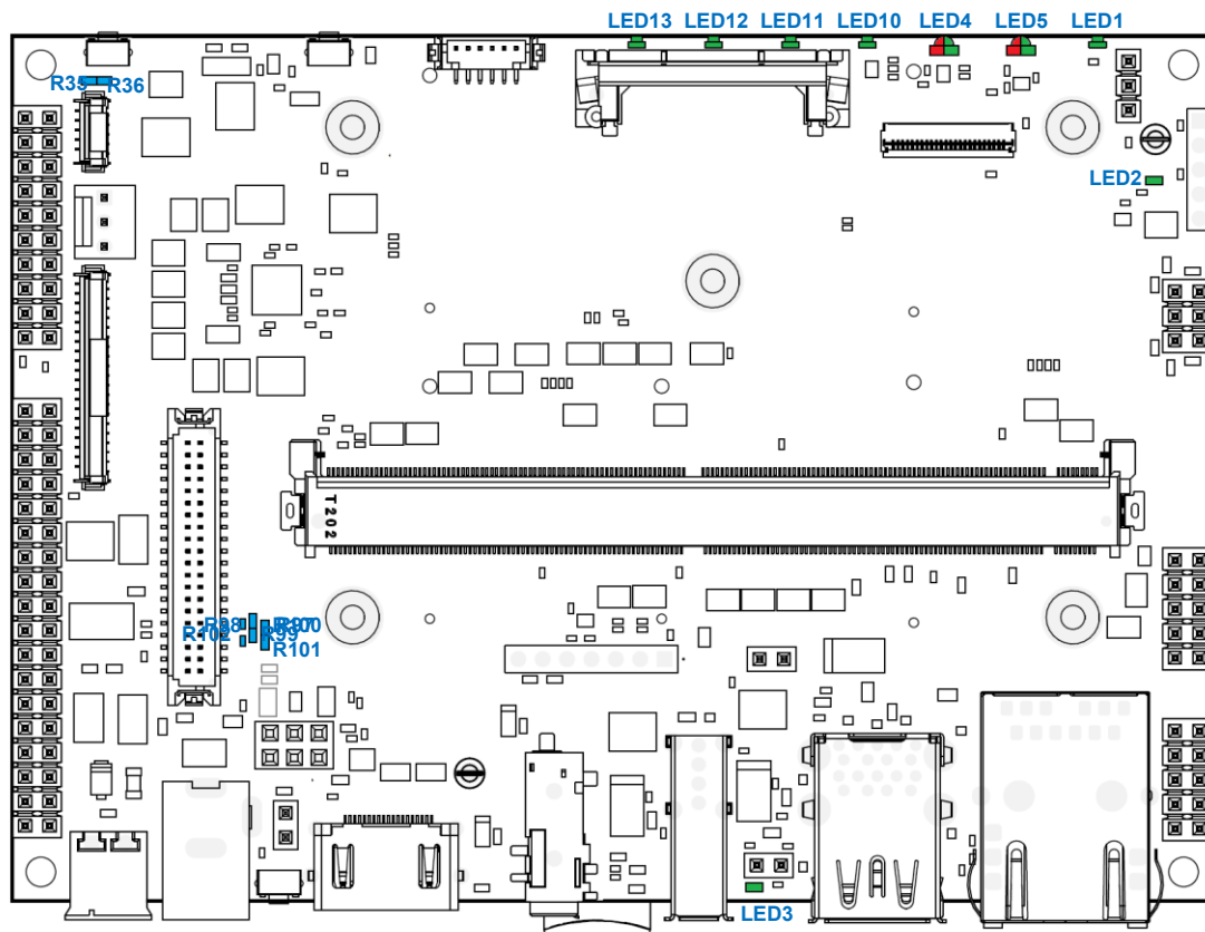
Fig.4 Ixora Carrier Board Assembly Options – Top Side
