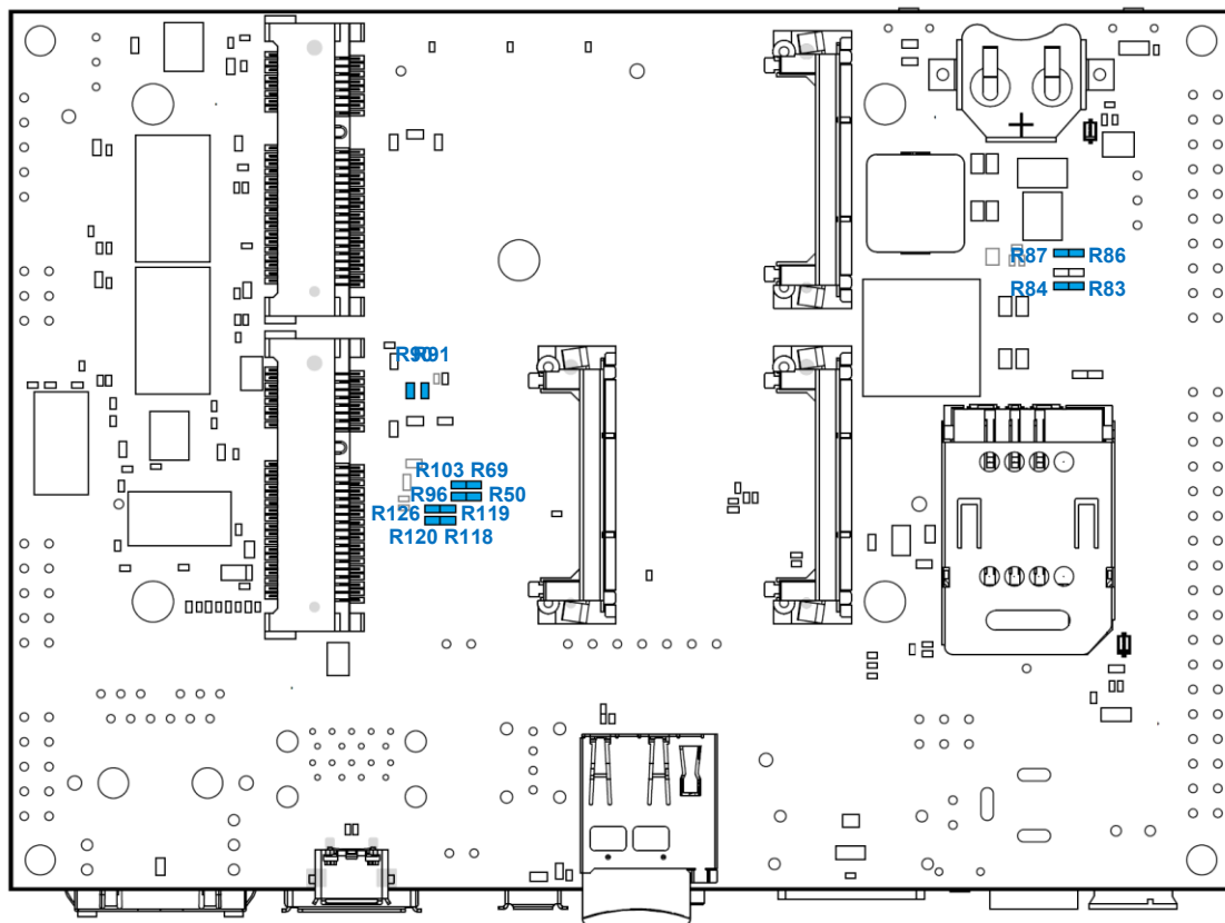
Fig.5 Ixora Carrier Board Assembly Options – Bottom Side
