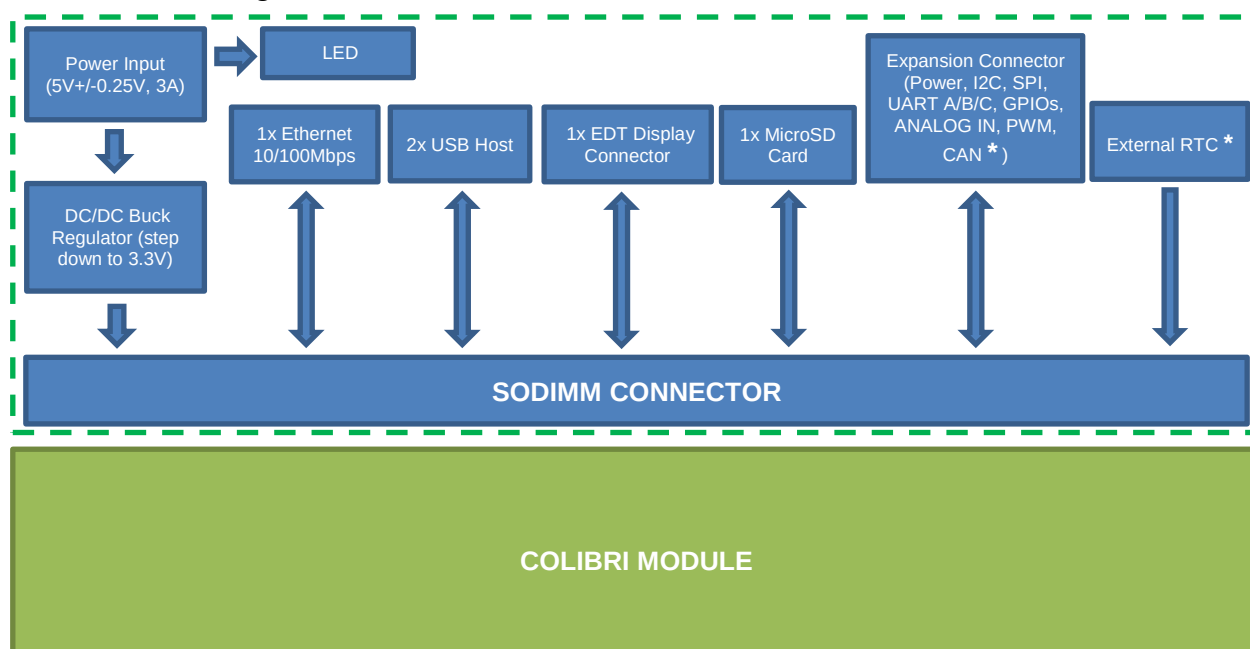
Fig. 1 Viola Block Diagram
