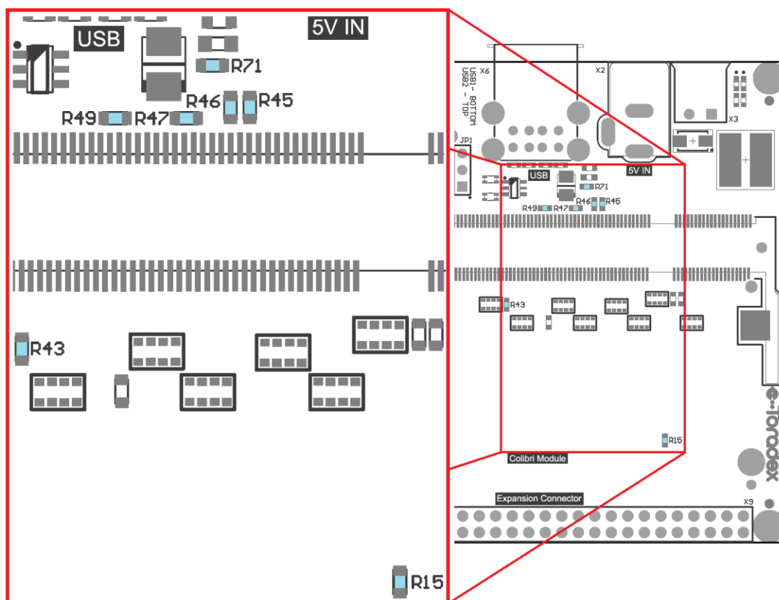
Fig.6 Viola Assembly Options – Top Side
