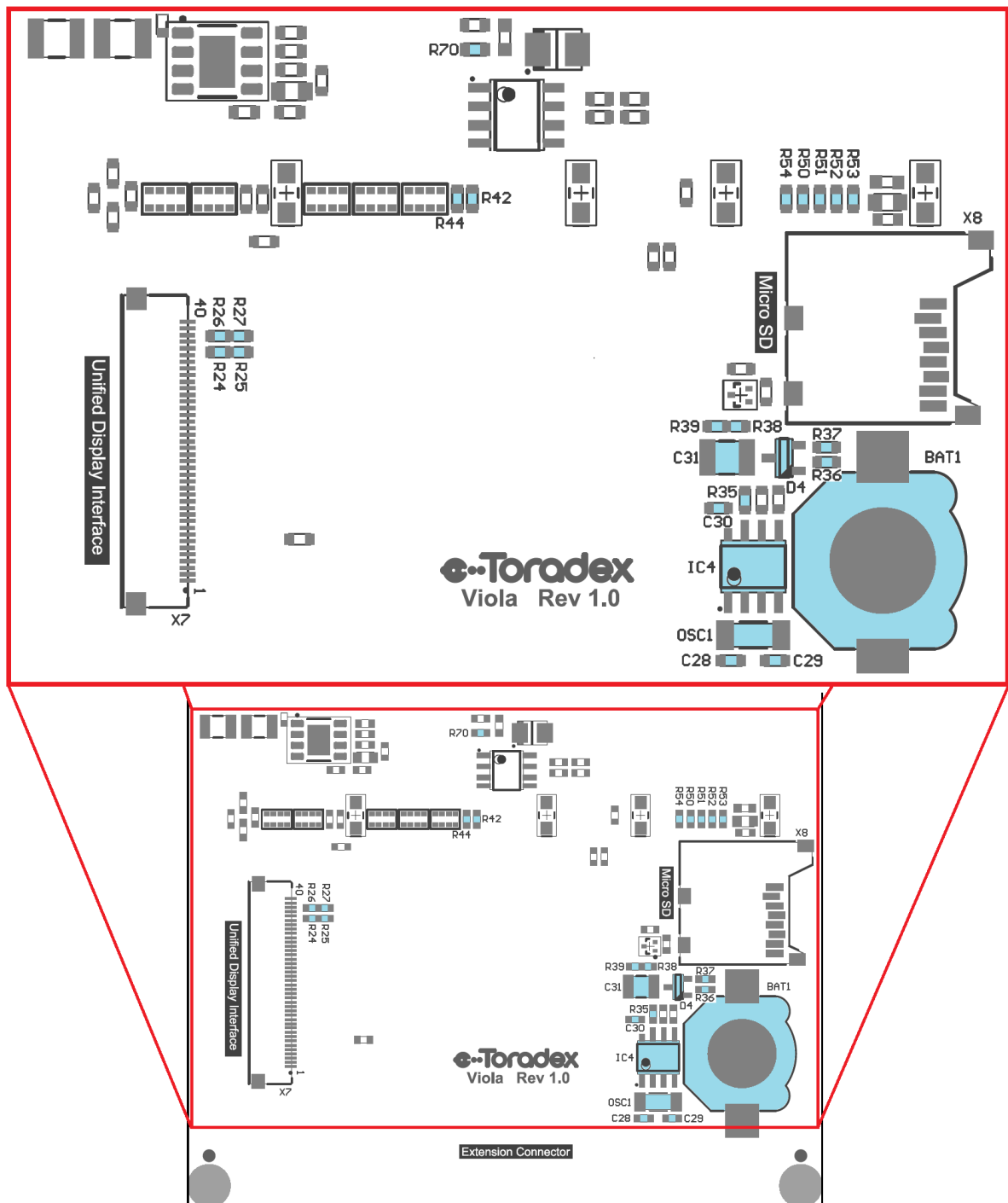
Fig.7 Viola Assembly Options – Bottom Side
