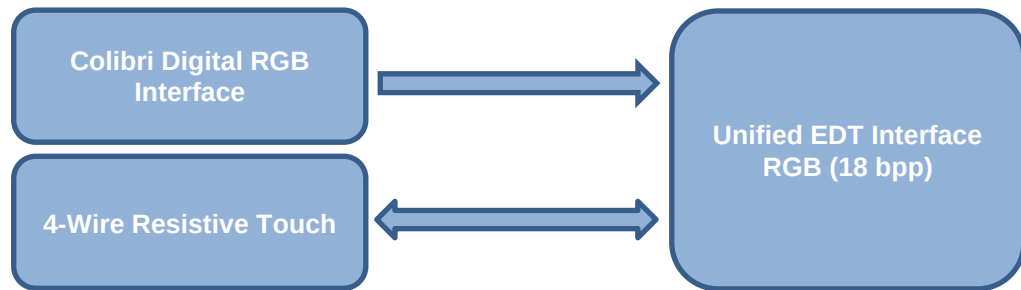
Fig.5 Display Interface Architecture
