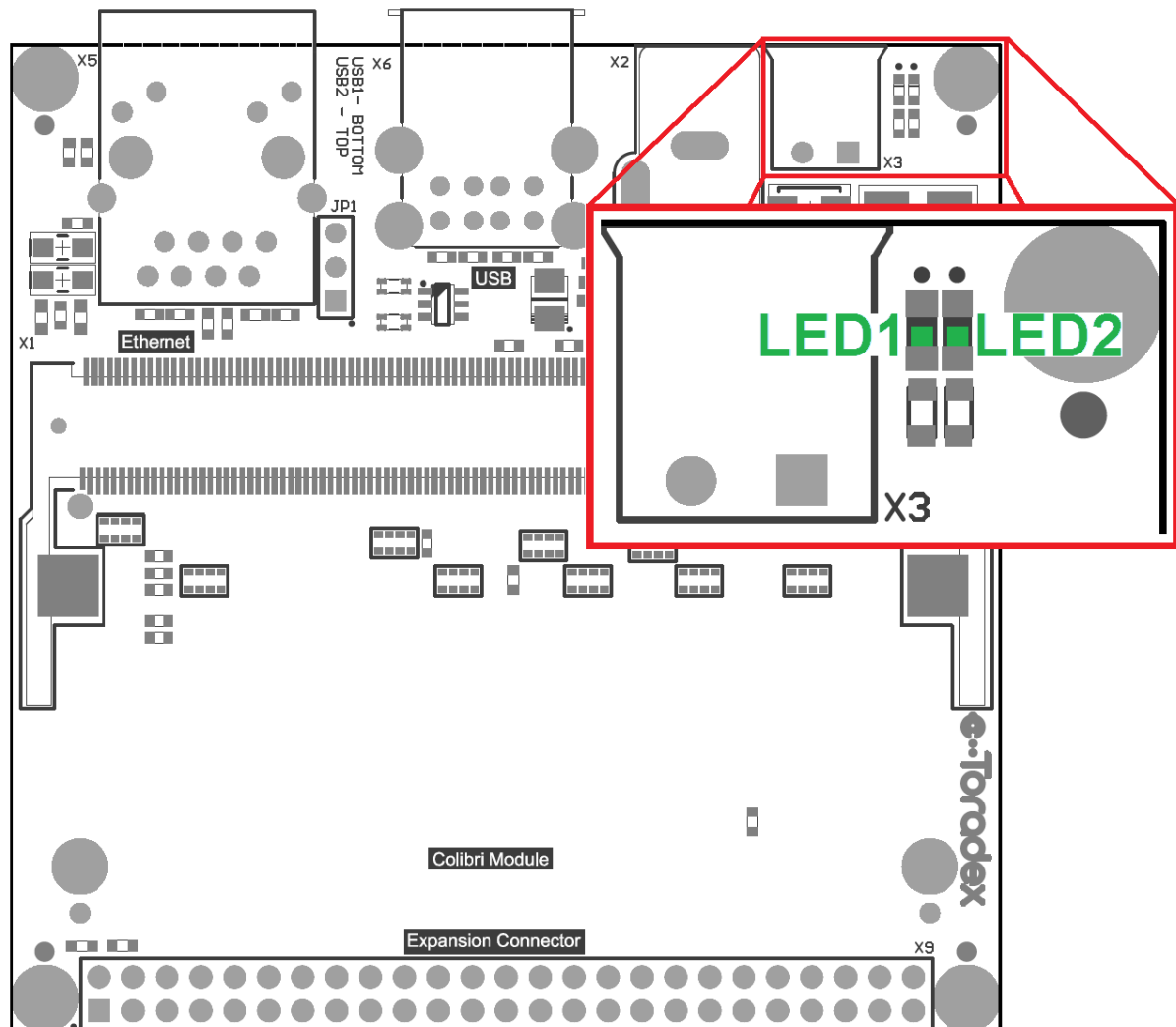
Fig.4 LED Positions
