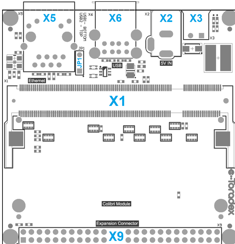
Fig.2 Viola connectors – Top Side
