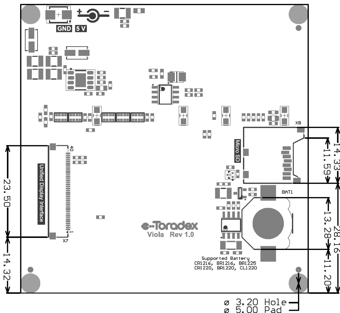
Fig.9 Viola Dimensions – Bottom Side, all dimensions are in millimetres (mm)
