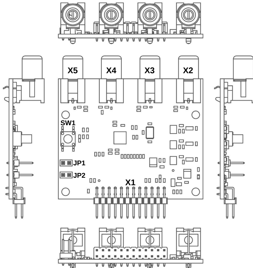
Fig.2 ACA Connectors – Top Side
