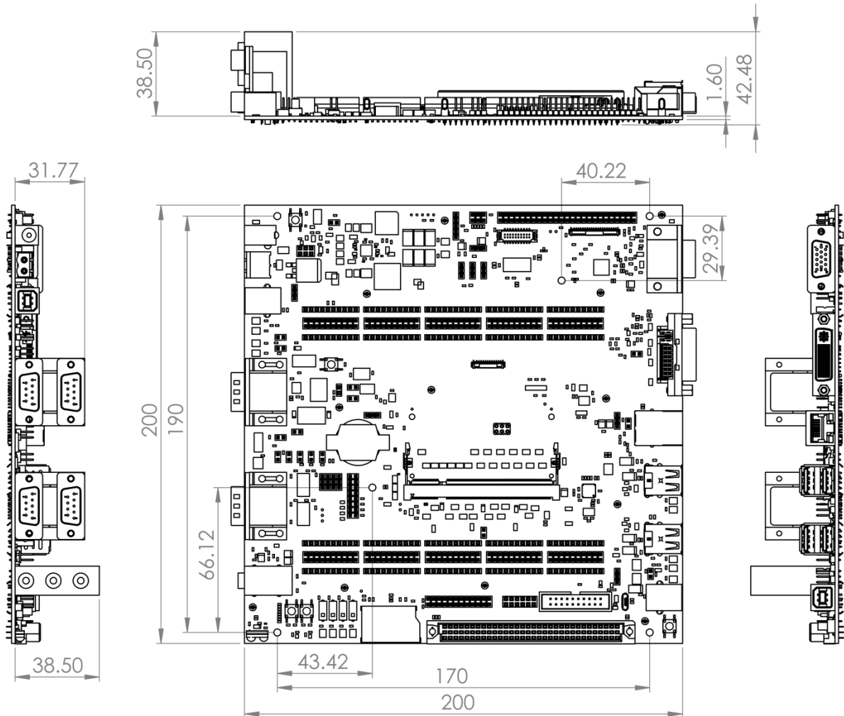
Fig.4 Colibri Evaluation Board Mechanical Drawing – Top Side
