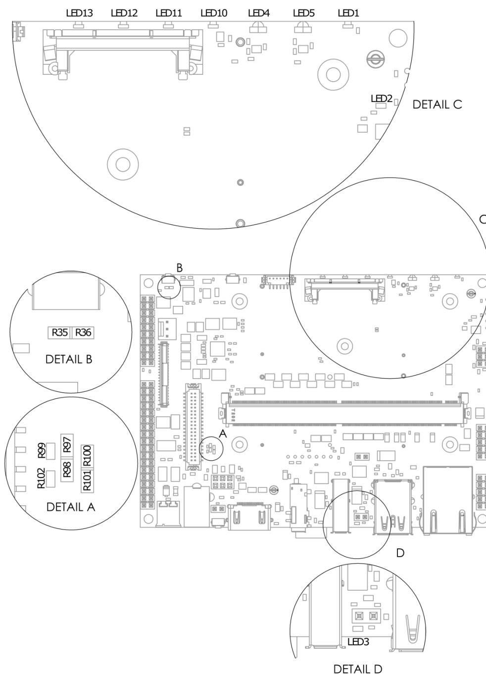
Fig.4 Ixora Carrier Board Assembly Options – Top Side
