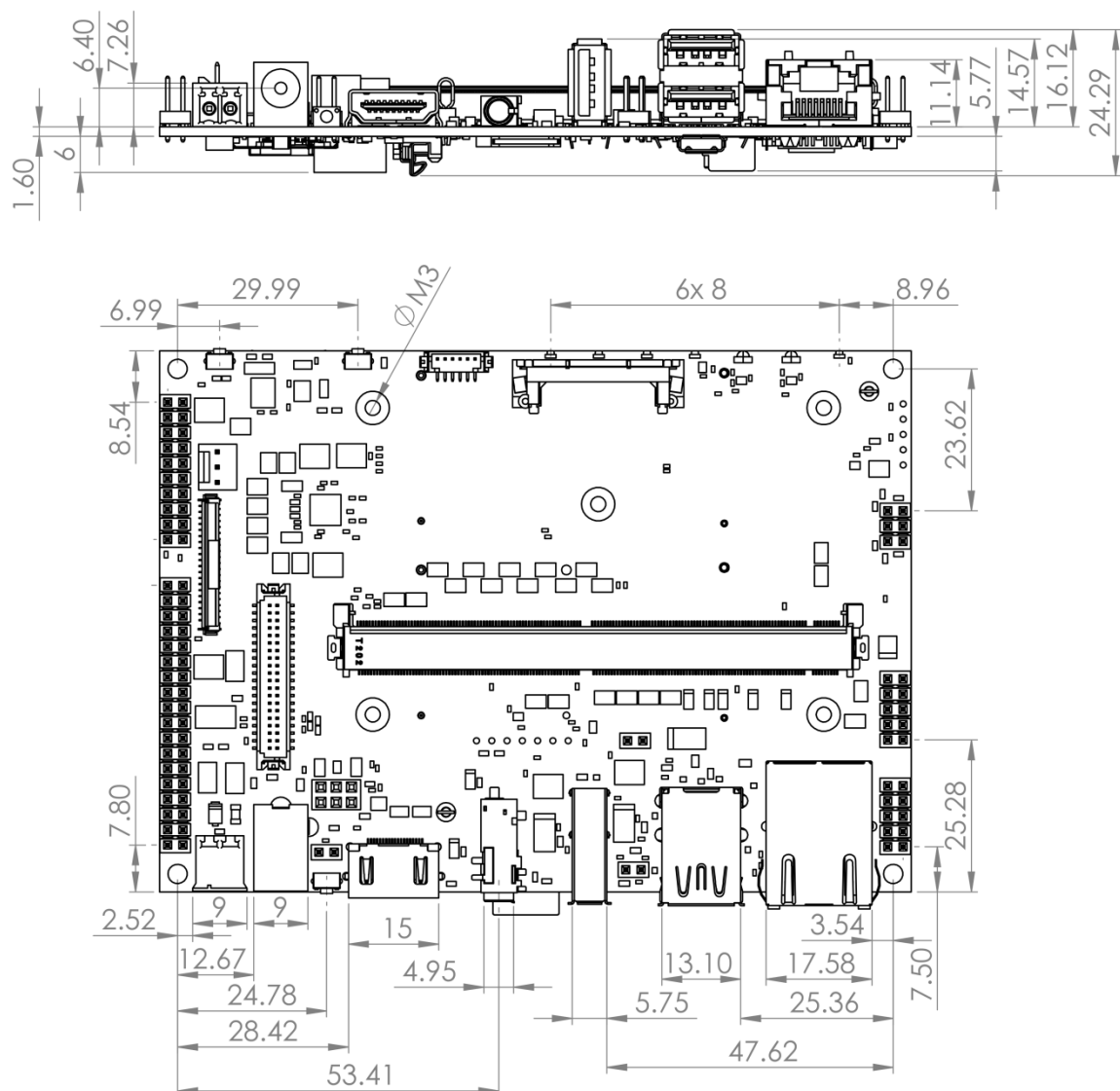
Fig.6 Ixora Carrier Board Mechanical Drawing – Top Side (All dimensions in millimeter)
