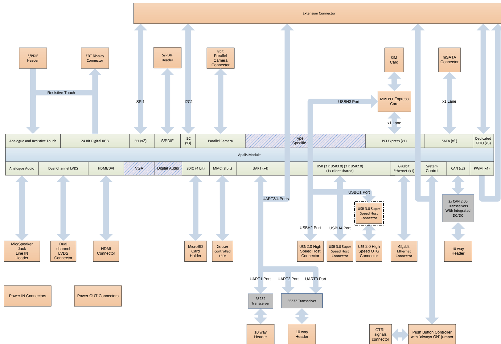
Fig.1 Ixora Carrier Board Hardware Architecture
