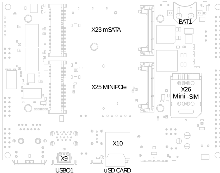
Fig.3 Ixora Carrier Board Connectors – Bottom Side
