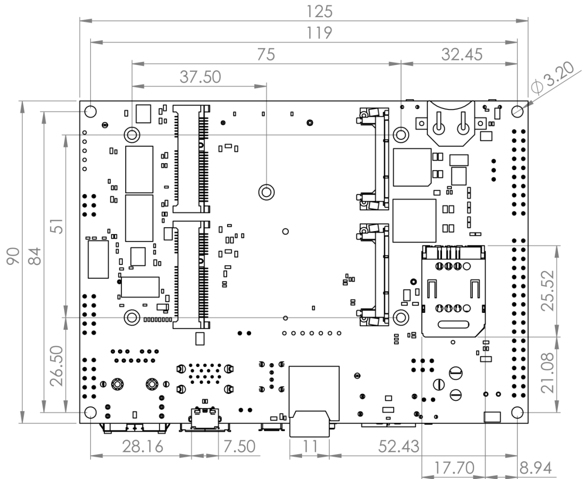
Fig.7 Ixora Carrier Board Mechanical Drawing – Bottom Side (All dimensions in millimeter)
