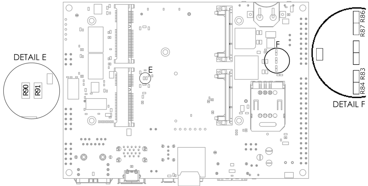
Fig.5 Ixora Carrier Board Assembly Options – Bottom Side
