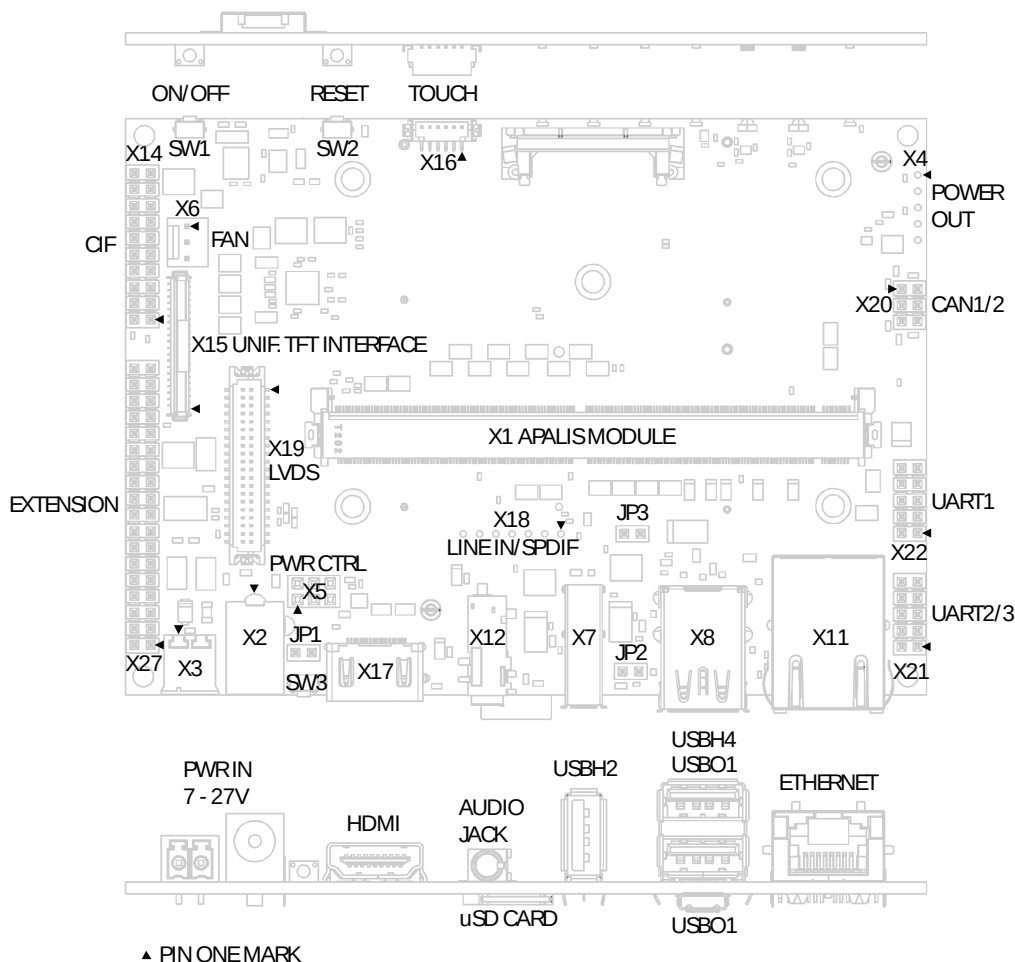
Fig.2 Ixora Carrier Board Connectors – Top Side
