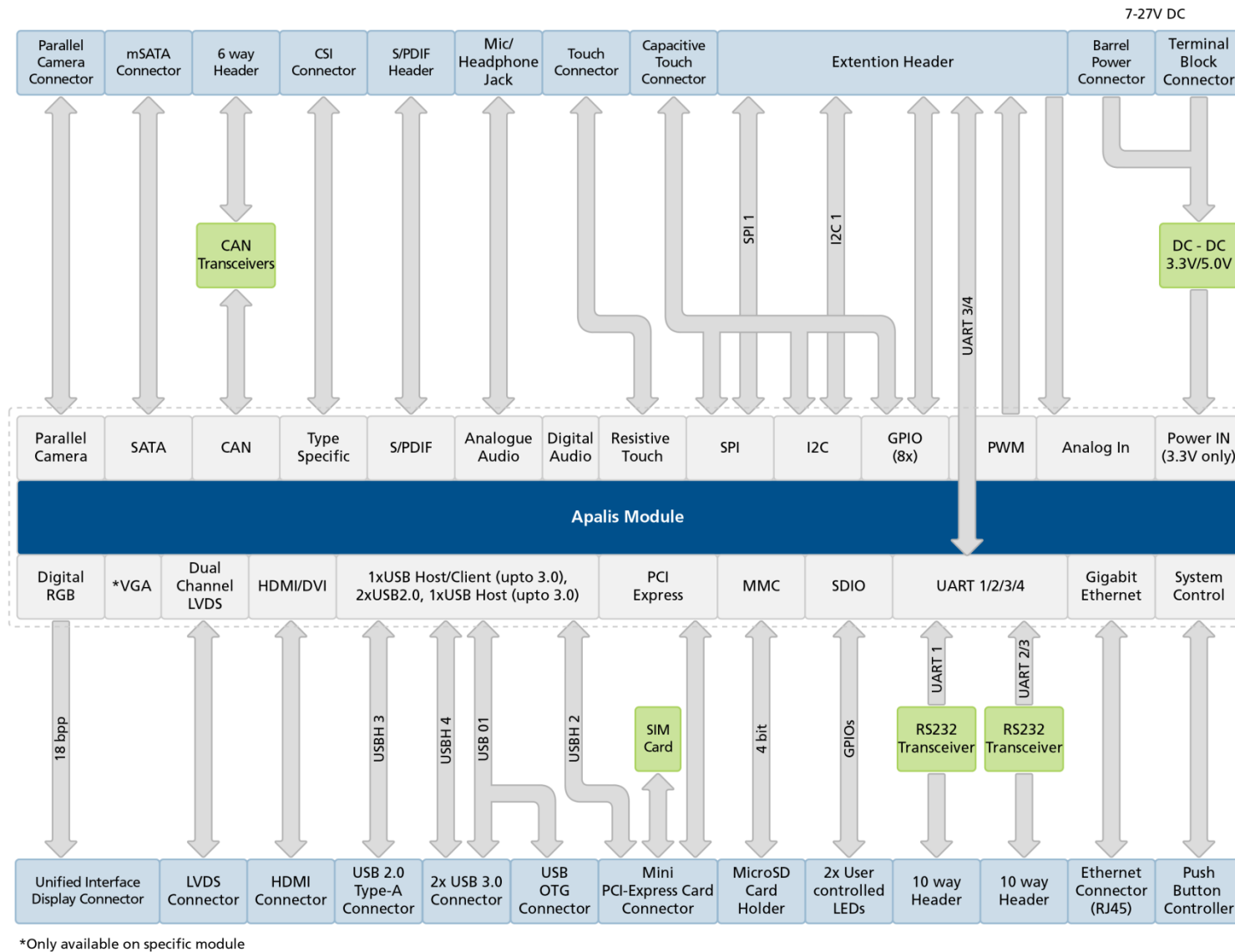
Fig.1 Ixora Carrier Board Hardware Architecture
