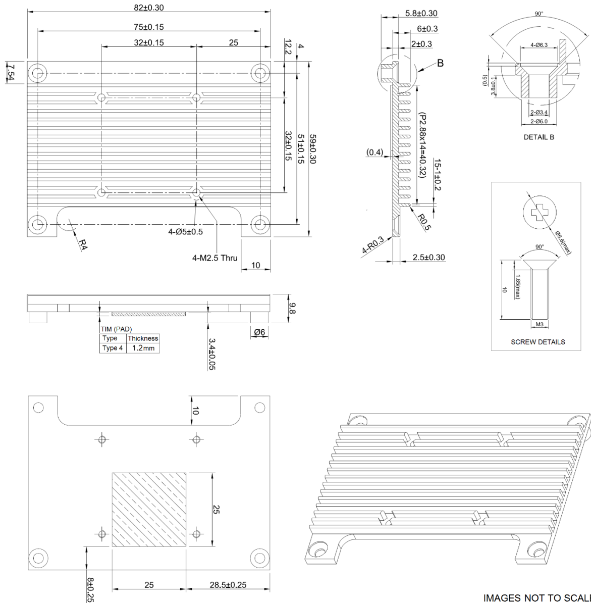
Figure 1-B: Apalis Heatsink Dimensions (Type-4)
