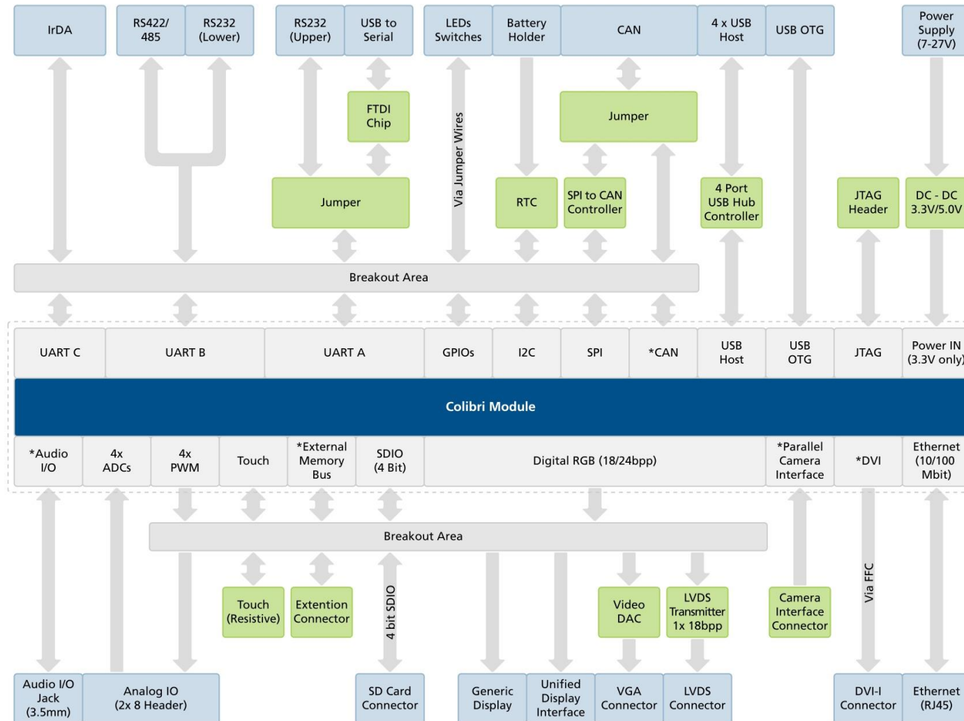
Fig.1 Colibri Evaluation Board Hardware Architecture
